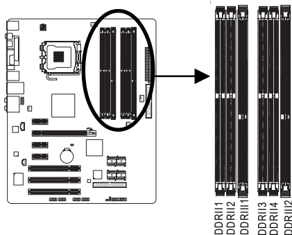
▶▶ DDR 2 Dual Channel Memory Configurations Table
