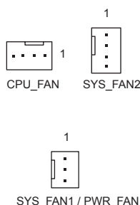
SYS_FAN1/PWR_FAN:
