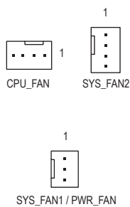
SYS_FAN1/PWR_FAN:
