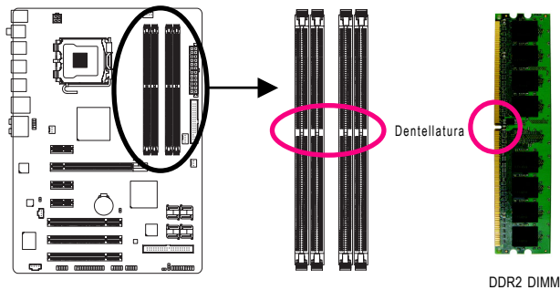
DDR2 DIMM
