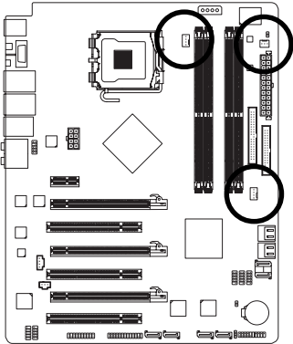
CPU_FAN / SYS_FAN
