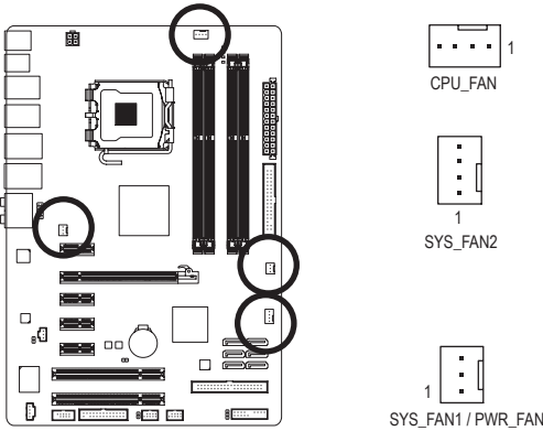
CPU_FAN:
