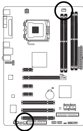
CPU_FAN
