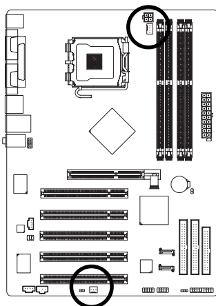
CPU_FAN
