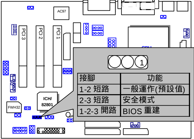
JP13 : 系統啟動方式選擇接腳 (Safe mode/Recovery/Normal)
