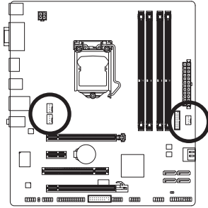
SYS_FAN1/SYS_FAN2
