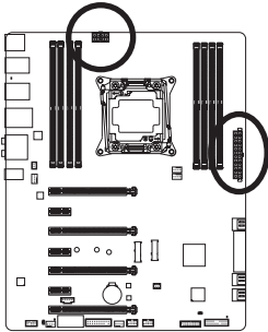
ATX_12V_2X4
