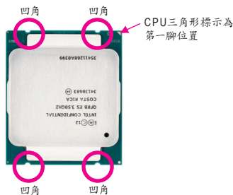
LGA2011-3 CPU
