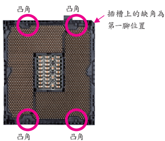
LGA2011 CPU
