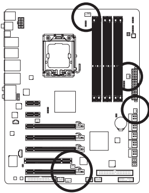
SYS_FAN1/PWR_FAN
