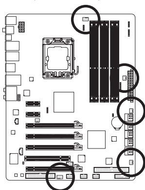
SYS_FAN1/SYS_FAN3/PWR_FAN
