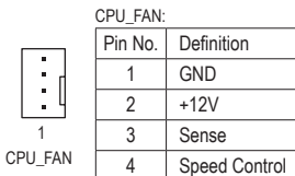
CPU_FAN
