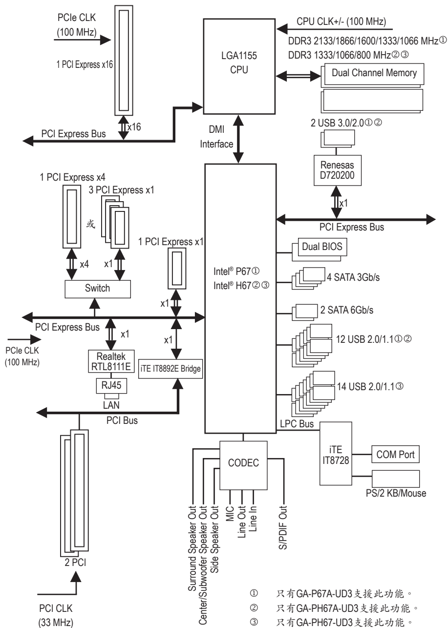
GA-P67A-UD3/GA-PH67A-UD3/GA-PH67-UD3主機板功能方塊圖
