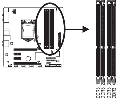
►► Dualchannel-Speicherkonfigurationstabelle
