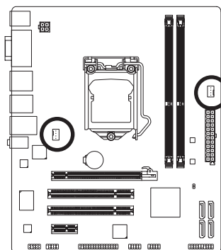
SYS_FAN
