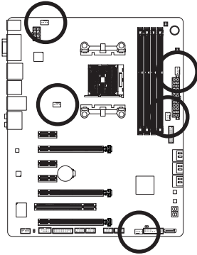
CPU_FAN SYS_FAN1
