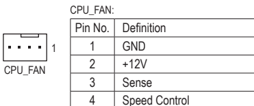
CPU_FAN:
