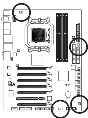
SYS_FAN2/PWR_FAN
